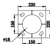
Anchor bolt
